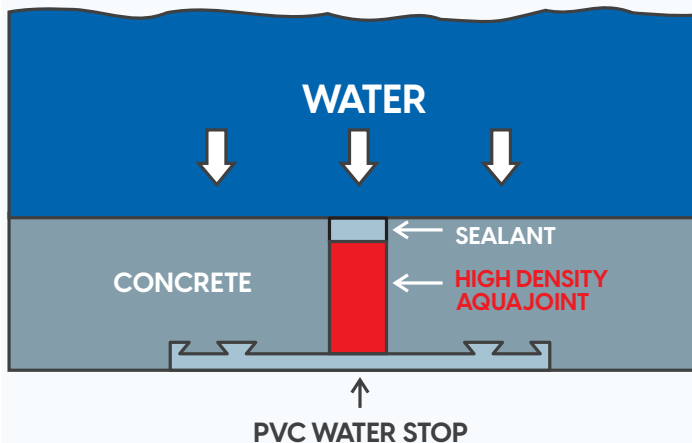
Side View of Water Retaining Structure
